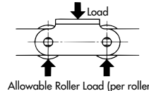
Base Chain Allowable Roller Load
