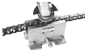
Figure 7: Grinding Down Pin Ends
