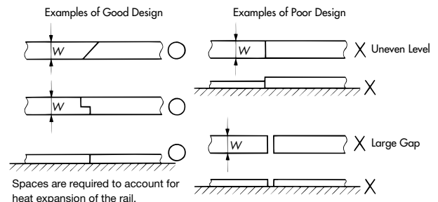
Figure 4: Rail Joints
